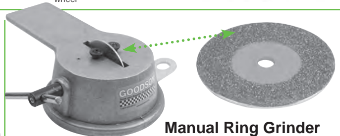
4 Table pivots past grinding wheel
