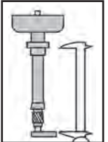
Fig. 4 Install adaptor in distributor drive. Measure as before and compare. Shim as needed to create clearance.
