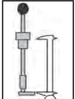
Fig. 3 Remove depth gauge from engine. Install adaptor in distributor tool. Measure and record depth.
